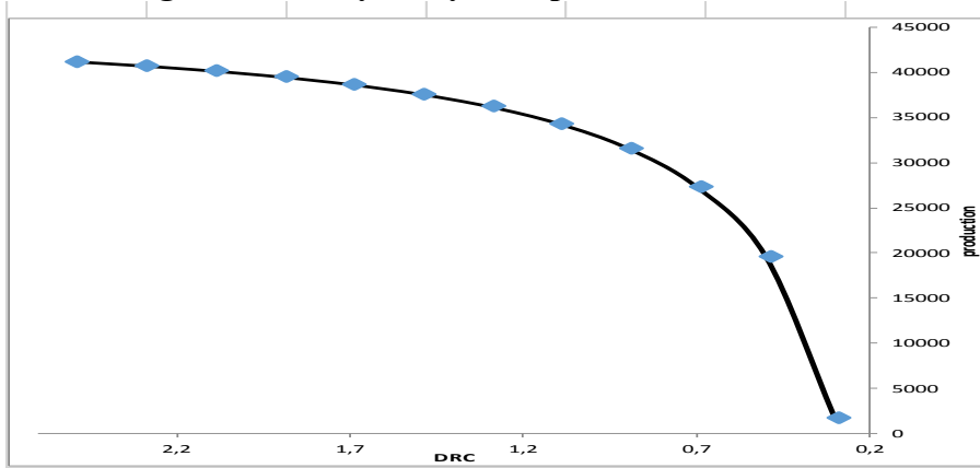
Fig.2. Sensitivity analysis of potato based on DRC
